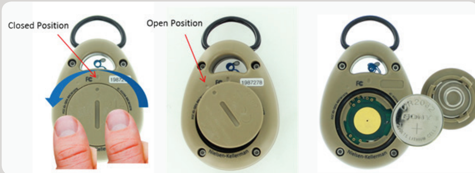
Figure 2: Battery Replacement
